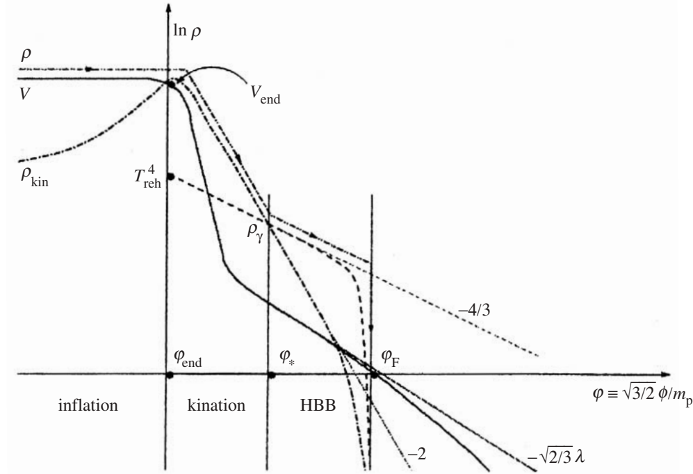
Figure 7.3 Schematic view of the scalar potential from inflation to quintessence. The potential V (solid line) features two flat regions, the inflationary plateau and the quintessential tail. The inflation is terminated at \varphi_{\text{end}} by a drastic reduction of V , leading to a rapid roll-down of the scalar field from the inflationary plateau towards the quintessential tail. At the end of inflation the kinetic energy density of the scalar field, \rho_{\text{kin}} (dash-dotted line), dominates for a brief period the energy density of the Universe. During this time the radiation energy density \rho_\gamma (dashed line) reduces less rapidly and catches up with \rho_{\text{kin}} at time t_* when the field is \varphi_* , and the explosive generation of entropy commences. After that the kinetic energy of the scalar field reduces rapidly to zero and the field freezes asymptotically to a value \varphi_F , while the overall energy density of the Universe (dash-dot-dotted line) continues to decrease due to the Hubble expansion. Assuming a quasi-exponential tail given by Equation (7.62), the potential beyond \varphi_F is seen departing logarithmically from a pure exponential case (dotted line). Reprinted from K. Dimopoulos and J. W. F. Valle, Modeling quintessential inflation [9], copyright 2002, with permission from Elsevier.
