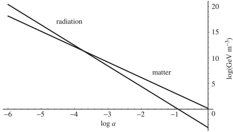
Figure 5.1 Scale dependence of the energy density in radiation \epsilon_r , which dominates at small a , and in matter \rho_m , which dominates at large a , in units of \log(\text{GeV m}^{-3}) . The scale value z_{\text{eq}} or a_{\text{eq}}^{-1} is evaluated in Equation (8.49) and indicated also in Figure 5.9.
