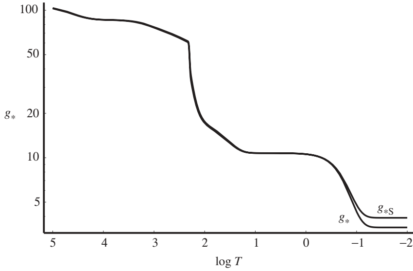
Figure 5.6 The evolution of the effective degrees of freedom contributing to the energy density, g_*(T) and to the entropy density, g_{*S}(T) , as functions of \log T , where the temperature is in units of MeV [4].
