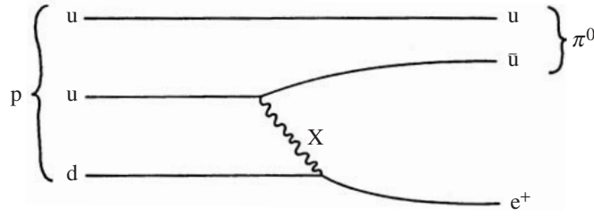
Figure 6.9 Proton decay Feynman diagram.
