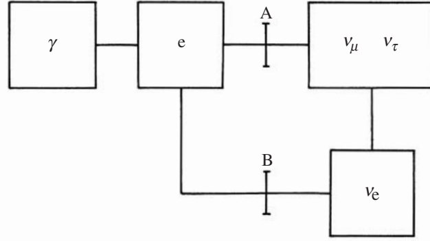
Figure 5.7 A system of communicating vessels illustrating particles in thermal equilibrium (from K. Kainulainen, unpublished research). At 3.7 MeV, valve A closes so that \nu_\mu and \nu_\tau decouple. At 2.3 MeV, valve B closes so that \nu_e also decouples, leaving only e^- and \gamma in thermal contact.
