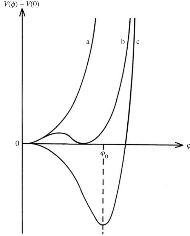
Figure 6.7 Effective scalar potentials. The different curves correspond to different temperatures. At the highest temperature (a) the only minimum is at \phi = 0 but, as the temperature decreases (b), a new minimum develops spontaneously. Finally, in (c), a stable minimum is reached at \phi_0 .
