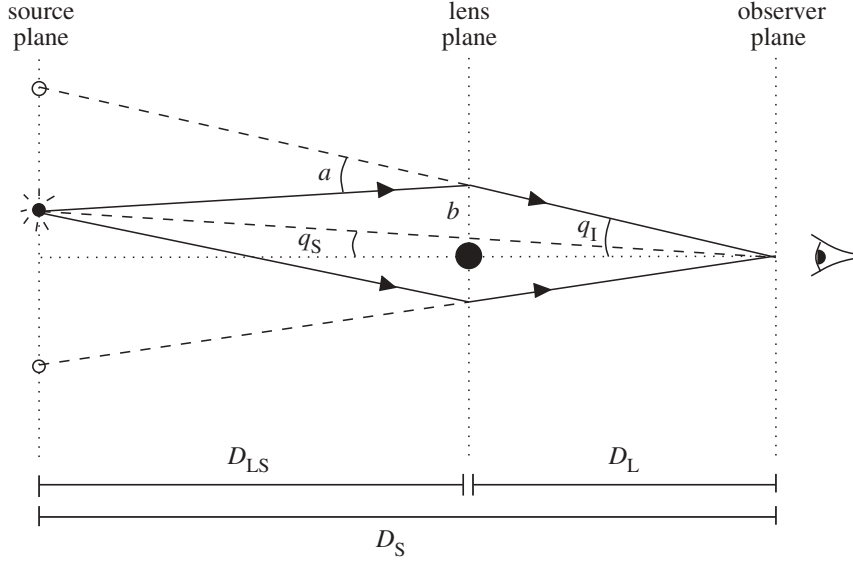
Figure 3.1 The geometry of a gravitational lensing event. For a thin lens, deflection through the small bend angle \alpha may be taken to be instantaneous. The angles \theta_1 and \theta_s specify the observed and intrinsic positions of the source on the sky, respectively. Reprinted from [4] with permission of J. A. Peacock.
