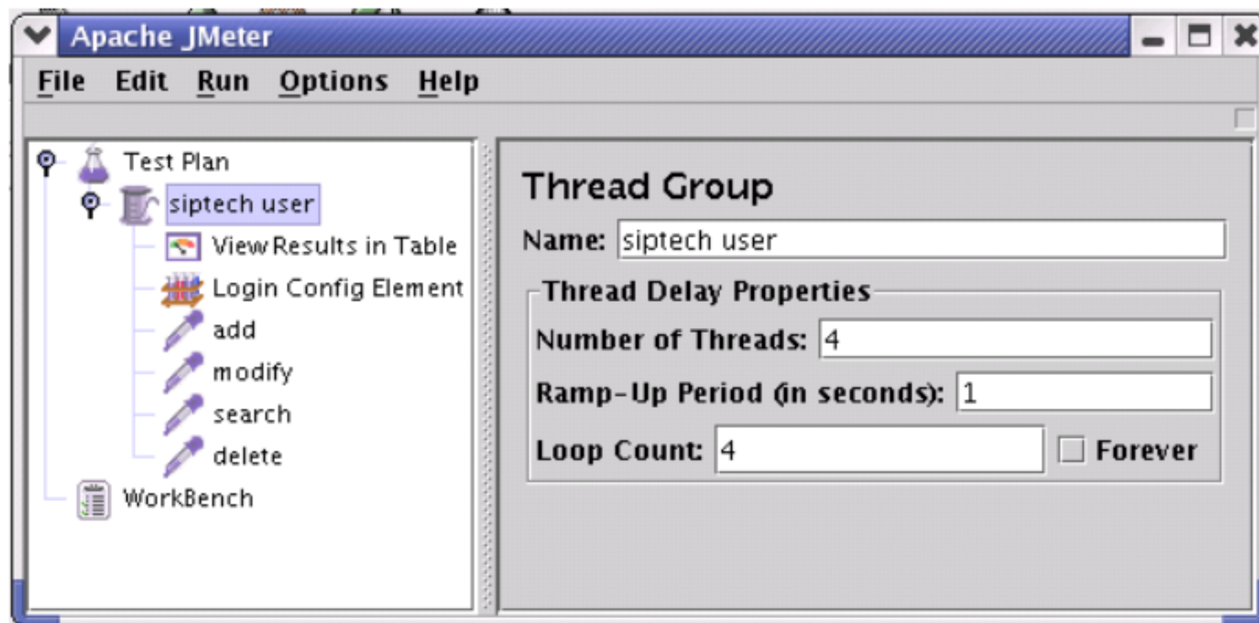
Figure 9.1. Thread Group with Default Values
