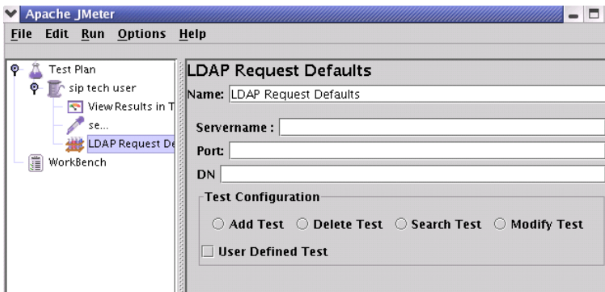
Figure 9.3 LDAP Defaults for our Test Plan
