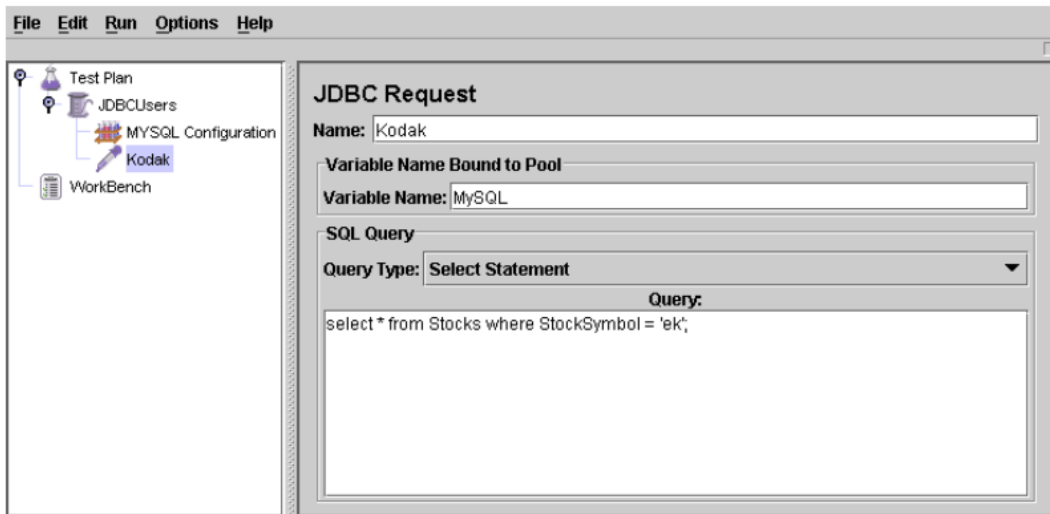
Figure 7.5. JDBC Request for Eastman Kodak stock
