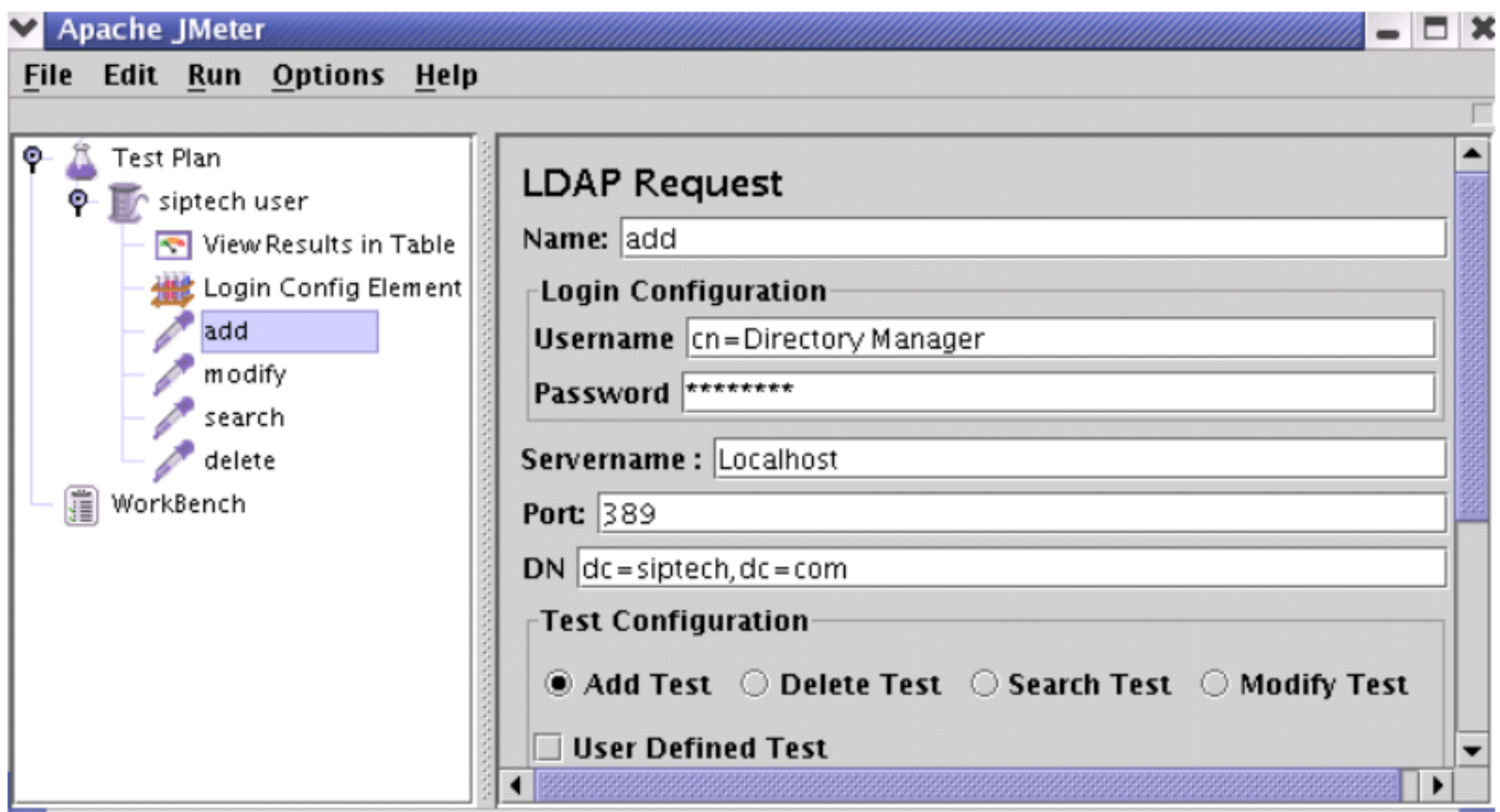
Figure 9.4.1 LDAP Request for Inbuilt Add test
