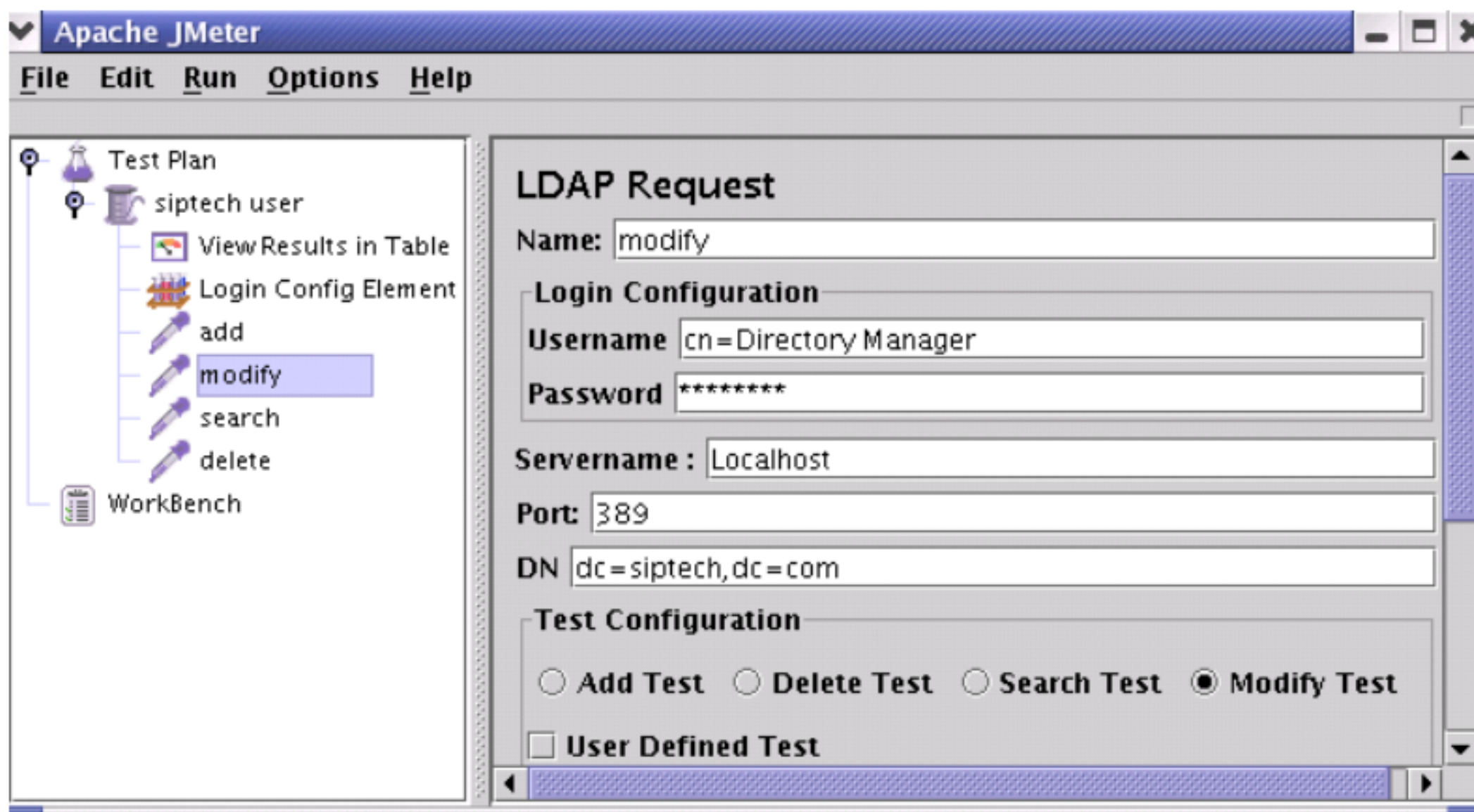
Figure 9.4.2 LDAP Request for Inbuilt Modify test
