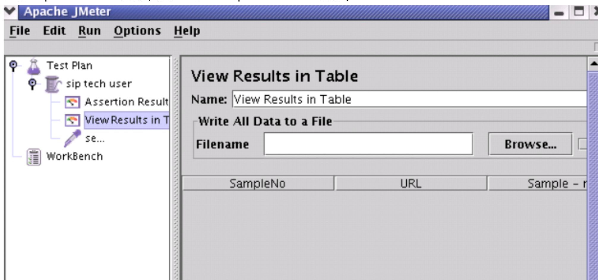
Figure 9.5 View result in Table Listener
