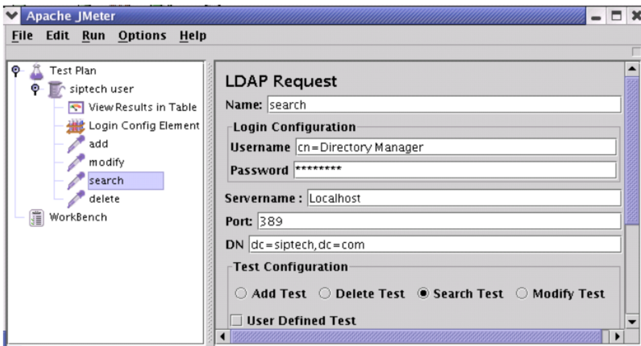
Figure 9.4.4 LDAP Request for Inbuilt Search test
