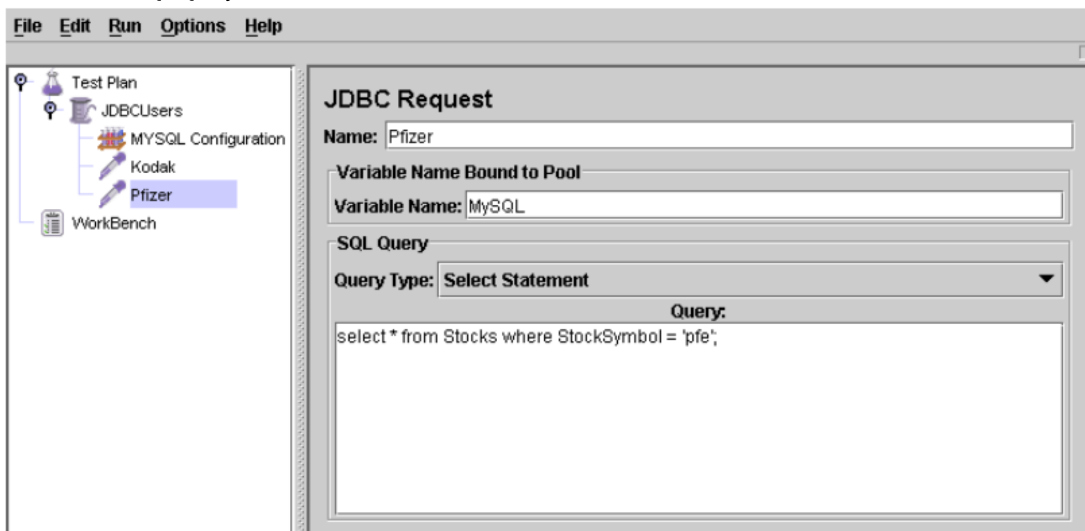
Figure 7.6. JDBC Request for Pfizer stock
