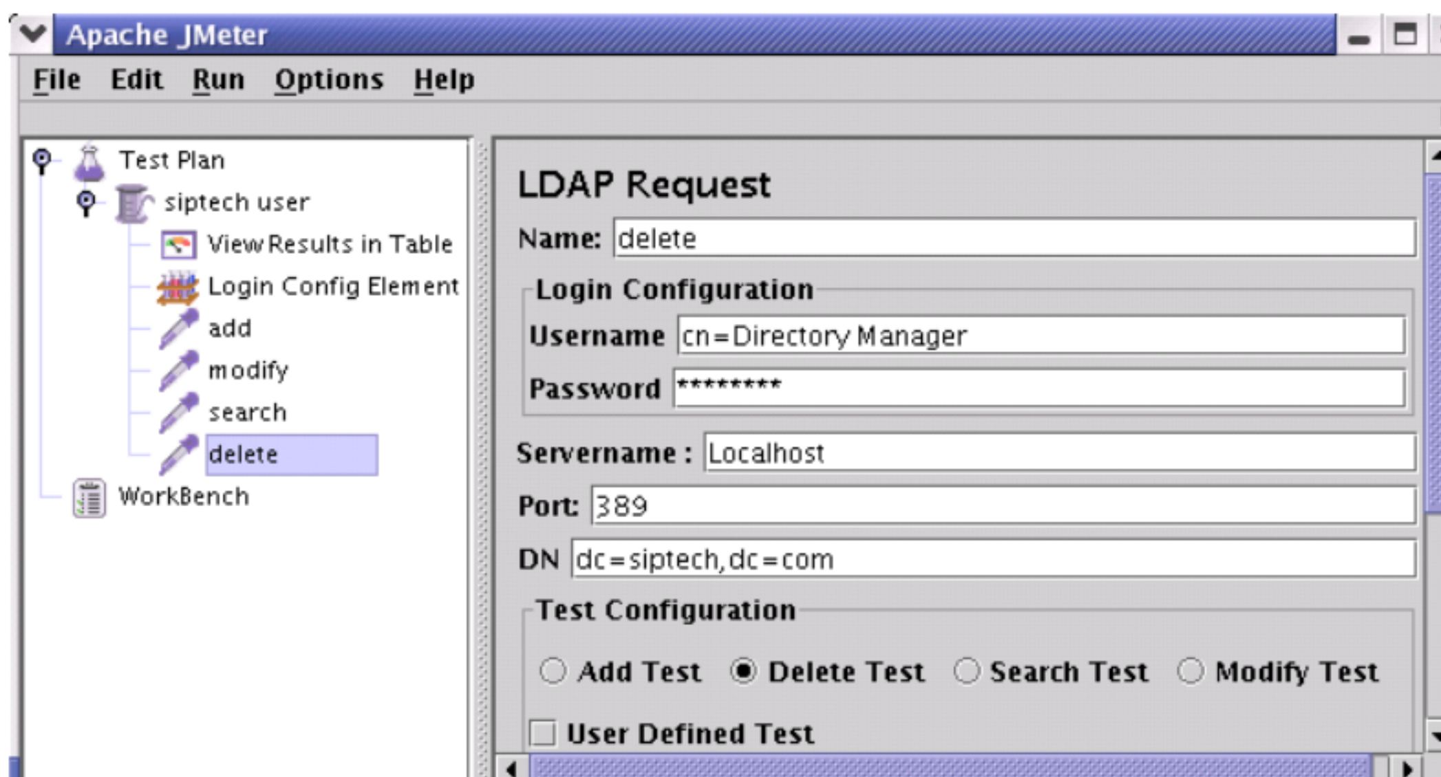
Figure 9.4.3 LDAP Request for Inbuilt Delete test
