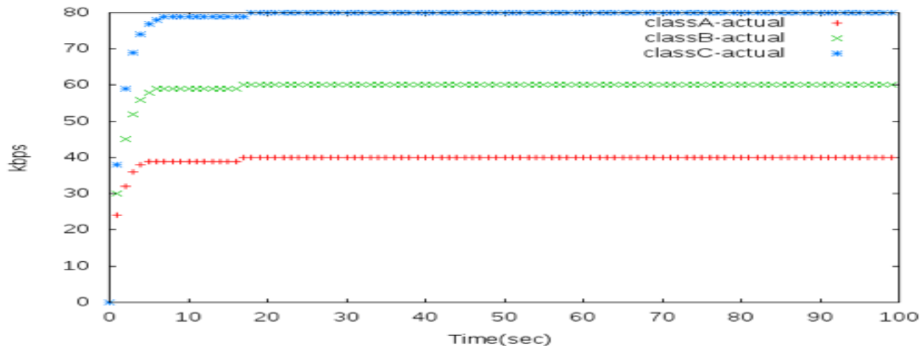
io-sched simulation
