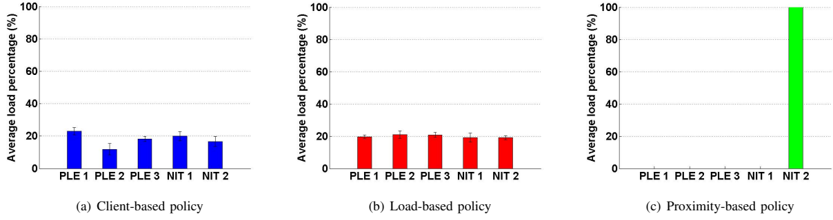
Fig. 4. Load balancing comparison among the three policies.
