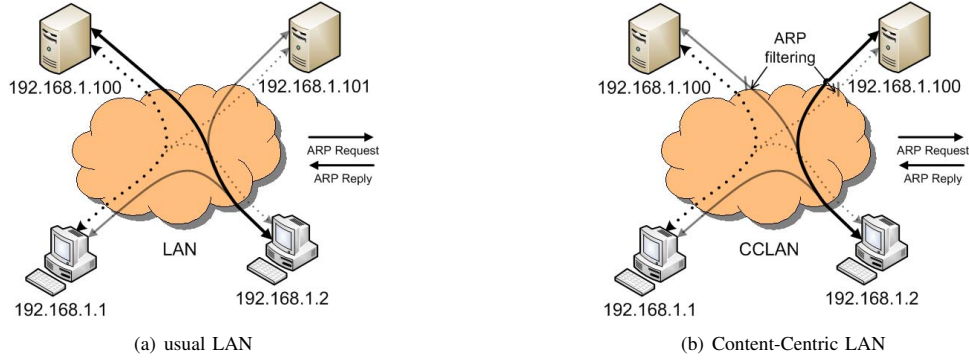
Fig. 1. The ARP messaging process in both cases of a usual LAN and a CCLAN. The dotted and solid lines correspond to the ARP Requests of .1 and .2 hosts respectively, for the .100 server. The bold lines indicate which ARP Request receivers answer with an ARP Reply.
