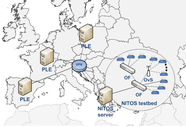
Fig. 3. European-wide single broadcast domain using a VPN connection.
